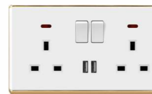
S2-057 2*13A switch socket+2USB w/without neon
